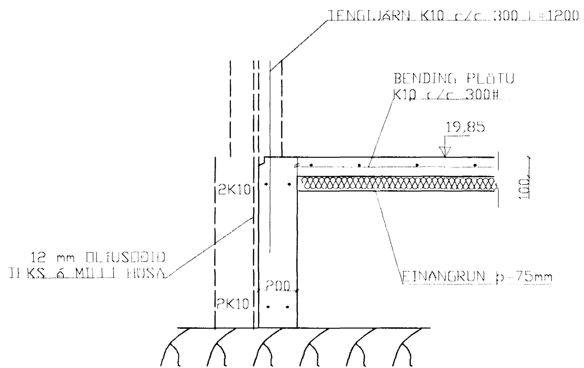
SNID 3, 1:20
