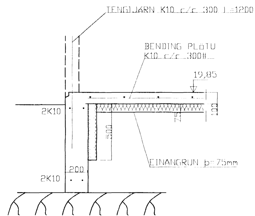
SNID 1, 1:20
