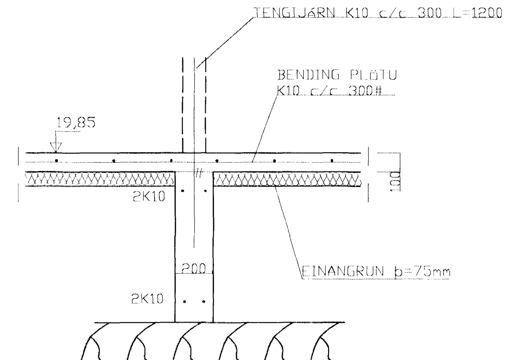
SNID 2, 1:20
