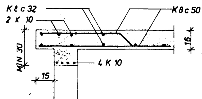
SNID A 1:20
