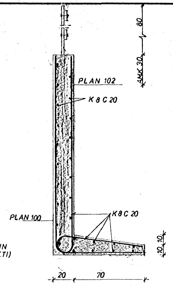
SNID 1:20
