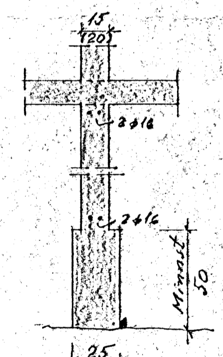
Snid B-B (C-C) 1:20
