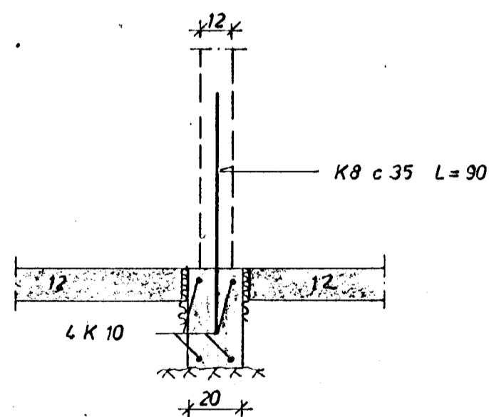
SNID B 1:20
