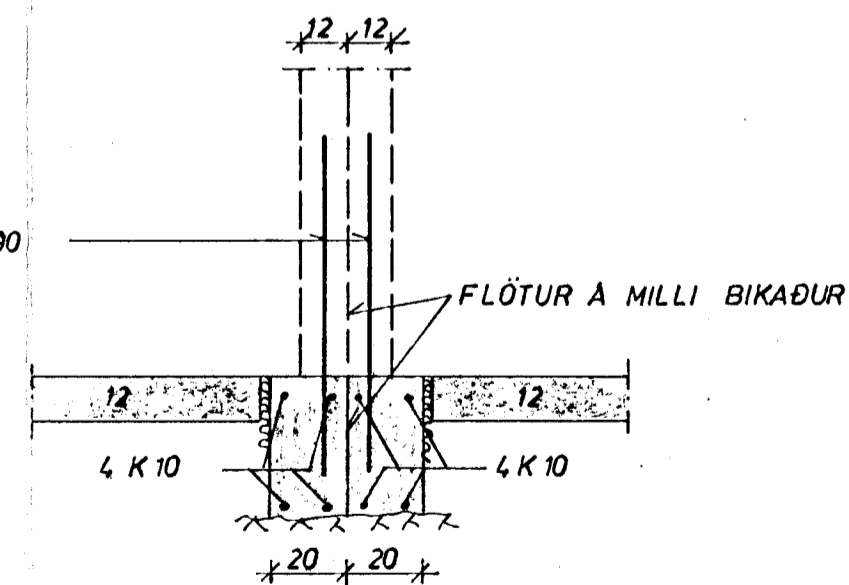
SNID C 1:20
