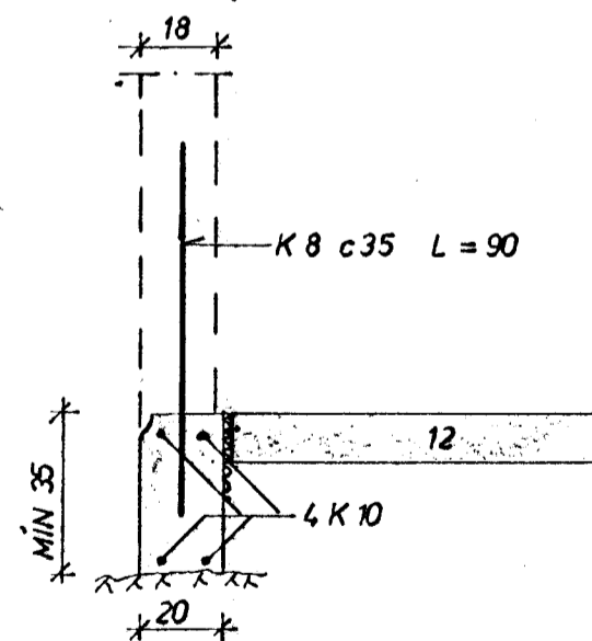
SNID A 1:20
