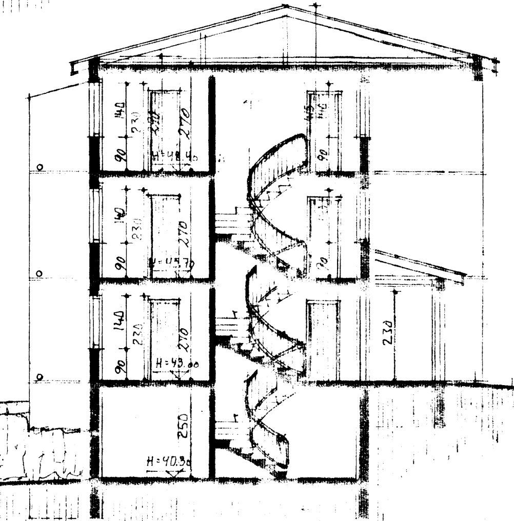
SNID B-B
