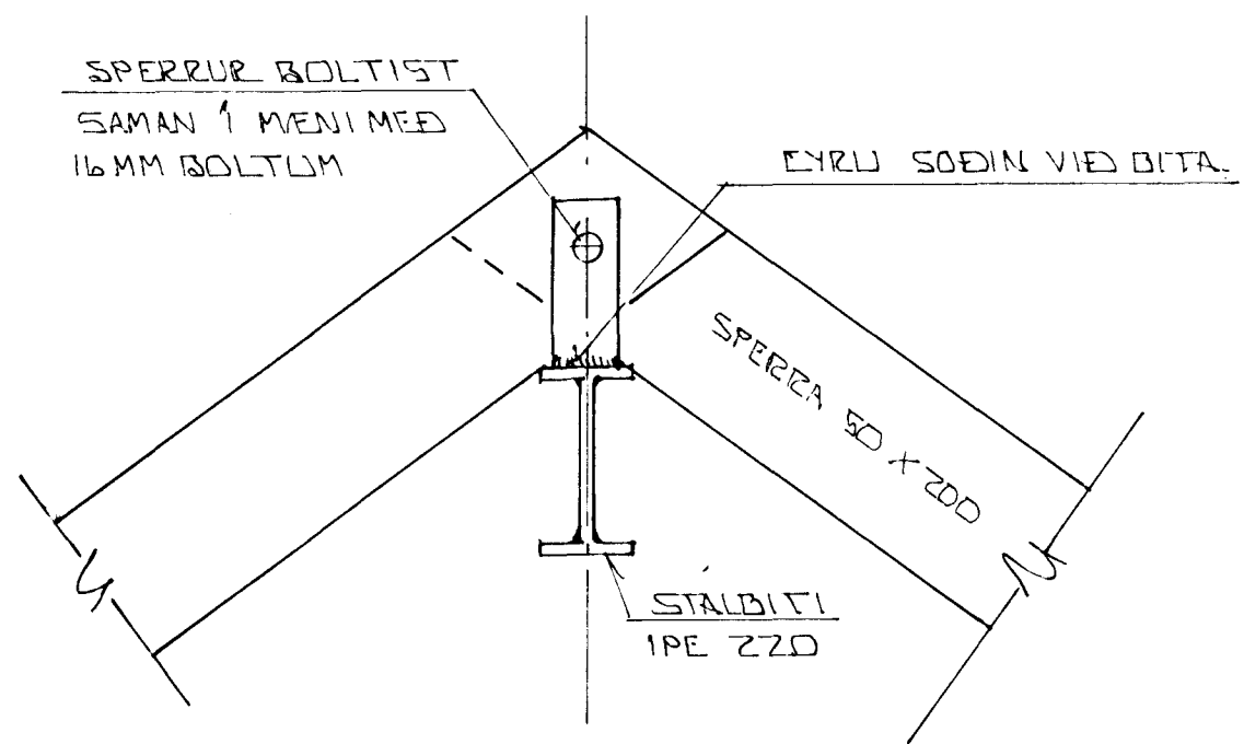
SNIED A - 1:10
