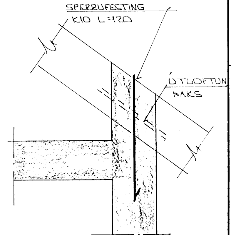
SNID C 1:20
