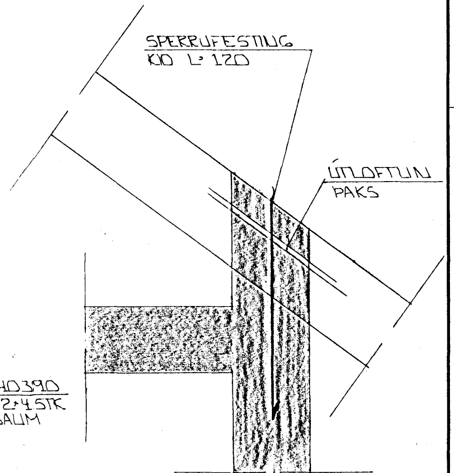
SNID 11 1:10
