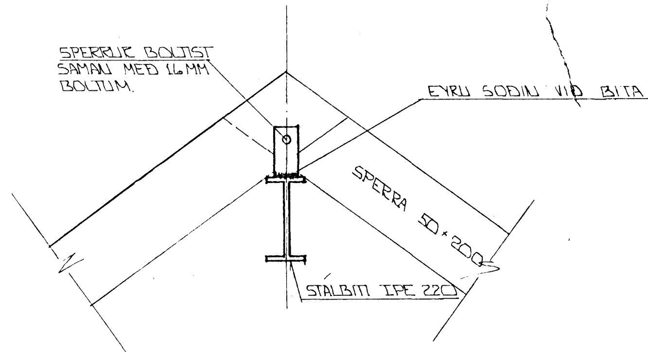
SNID 10 1:10
