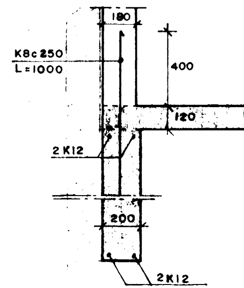
SNID B05 1:20
