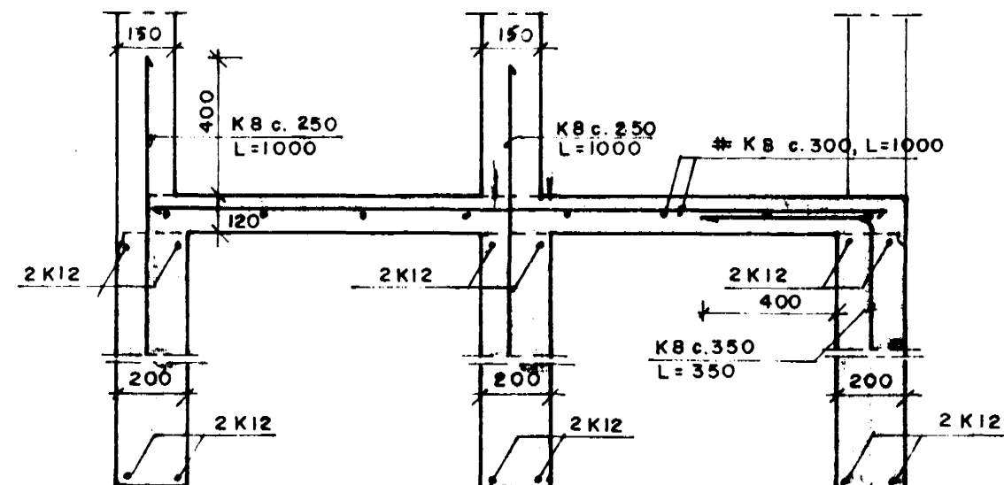
SNID F05 1:20
