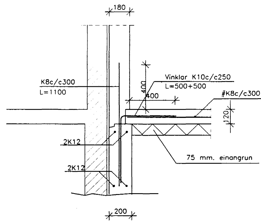
SNID B05 1:20
