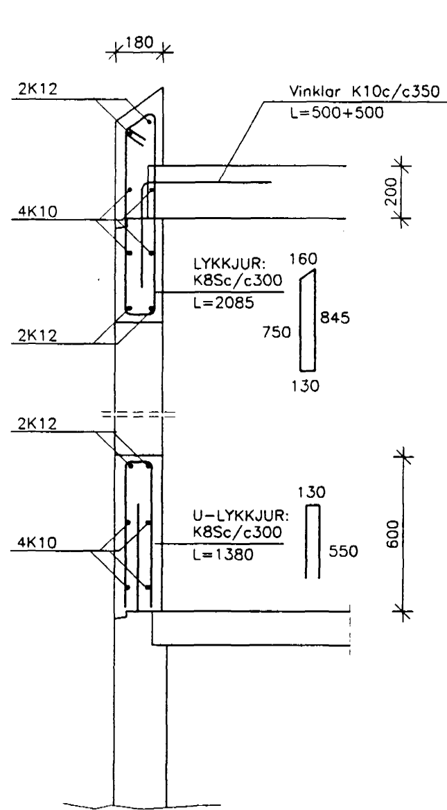
SNID B07 1:20
