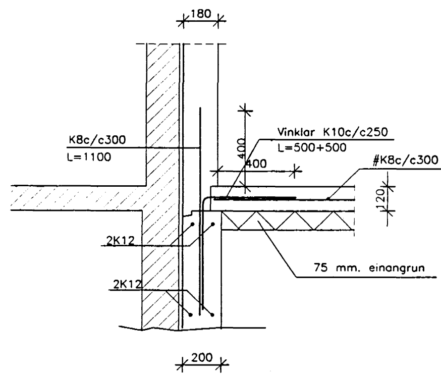
SNID B05 1:20
