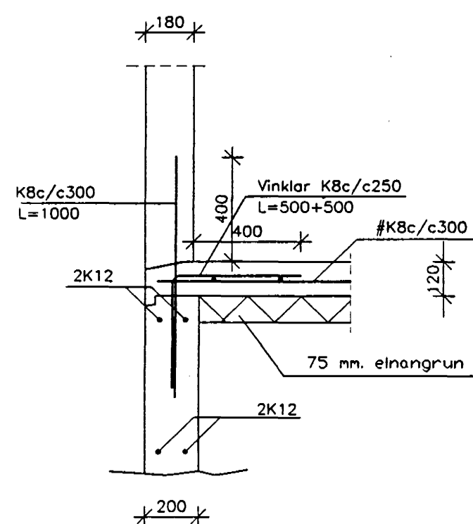
SNID F05 1:20
