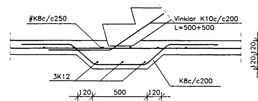
SNID G05 1:20
