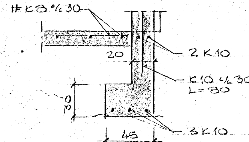
SNIP H 1:20
