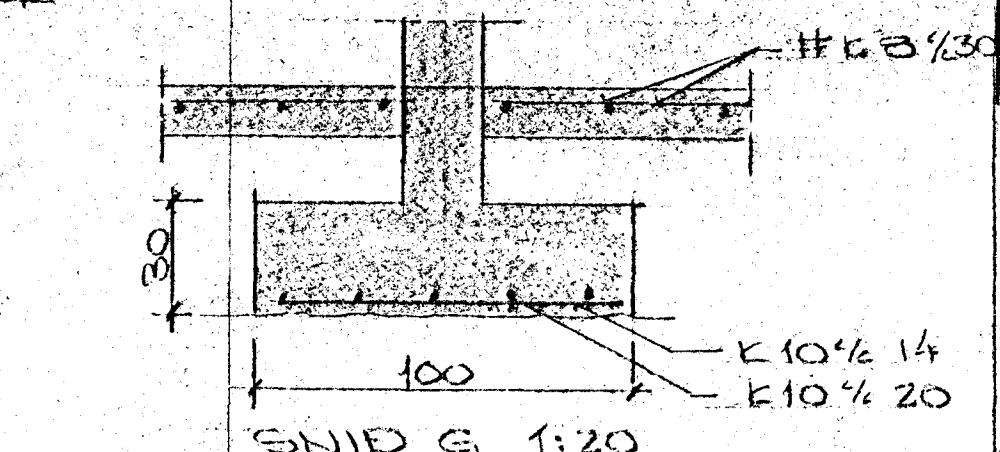
SNIP G 1:20
