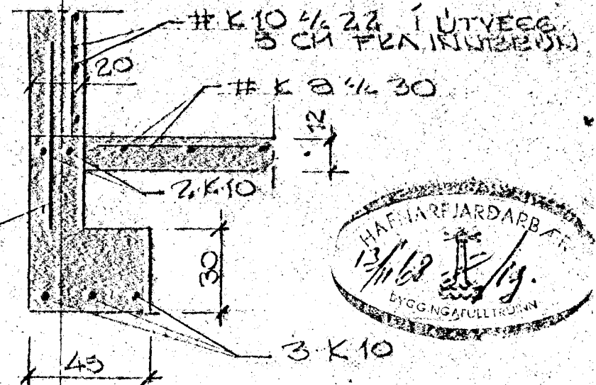
SNIP B 1:20
