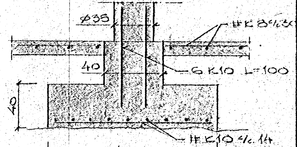
SNIP F 1:20
