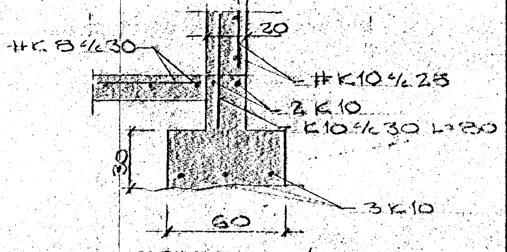
SNIP E 1:20
