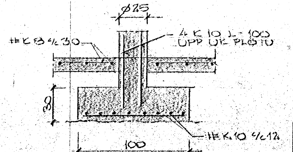
SNIP D 1:20
