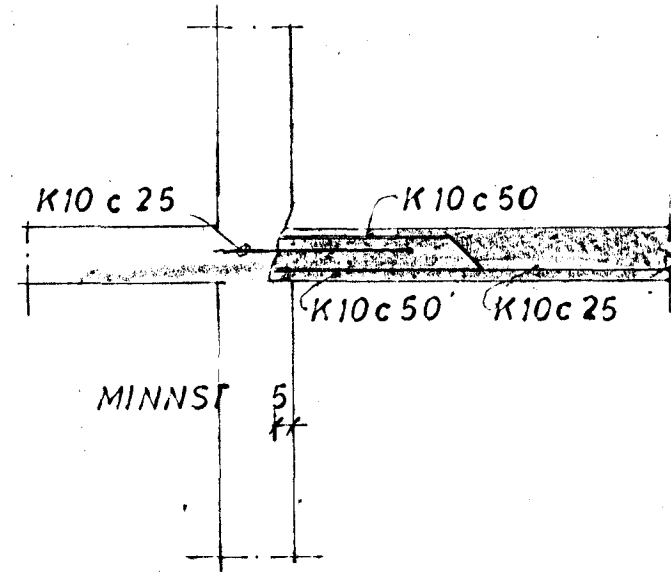
SNID B 1:20
