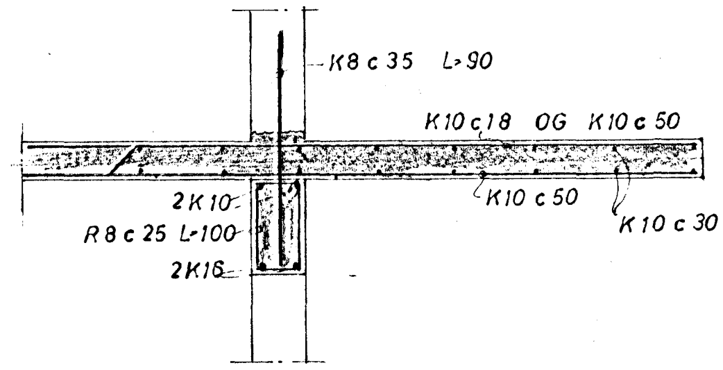
SNID C 1:20
