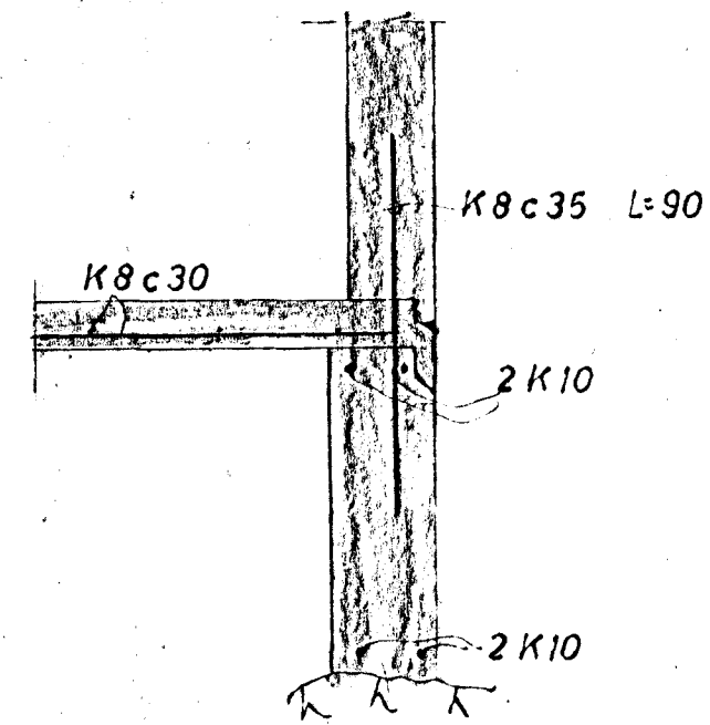
SNID A 1:20
