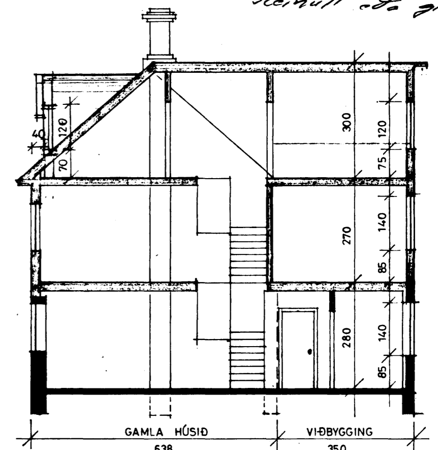
SNID 1:100
