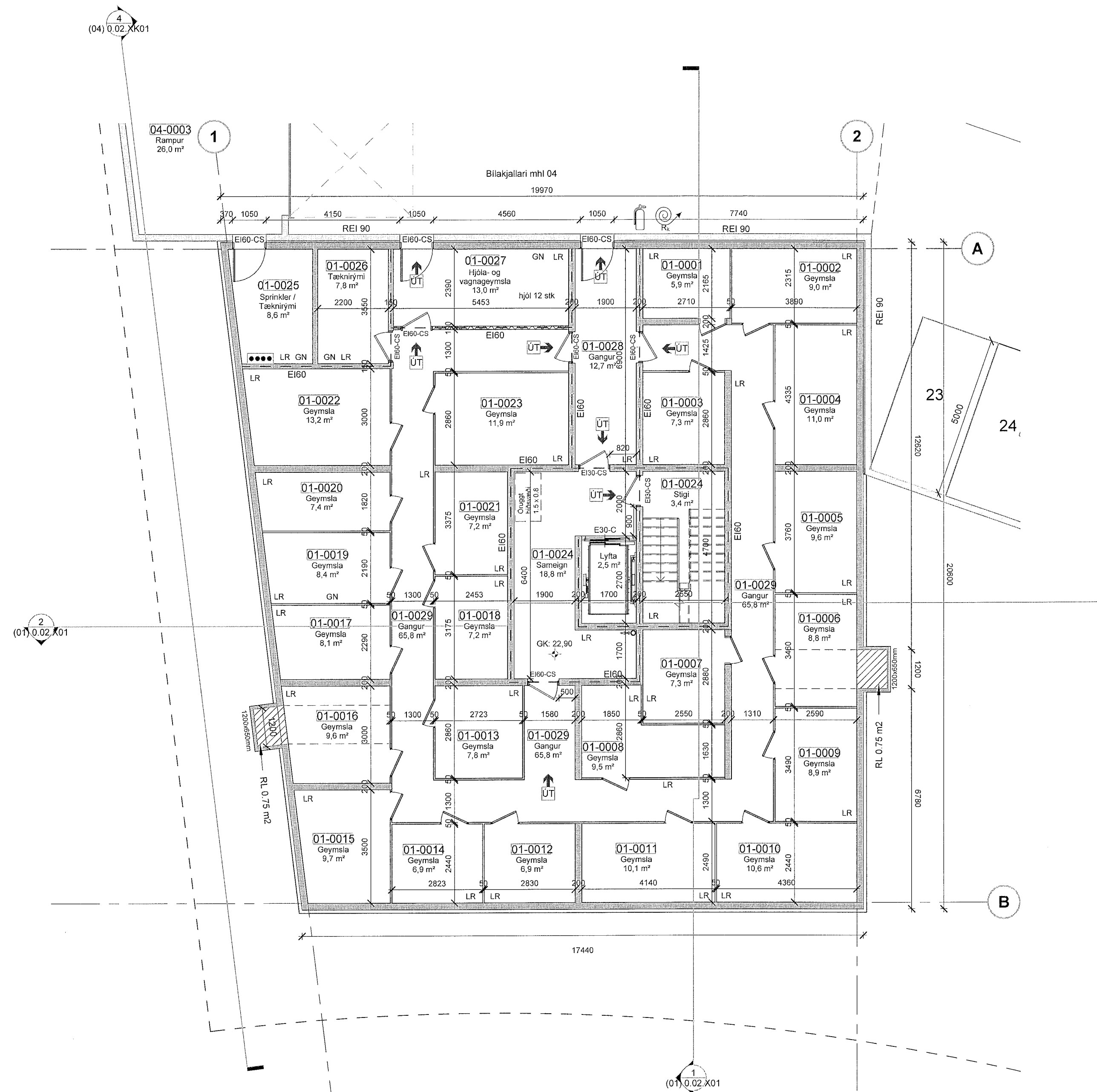
00-Kjallari - mhl 1 1: 100
