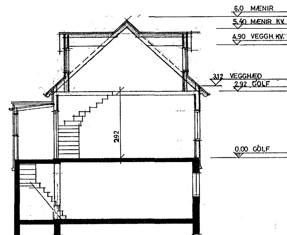
SNID 1:100
