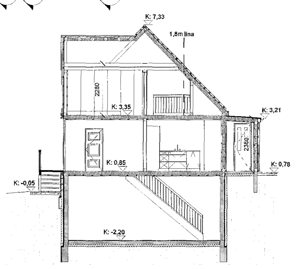
SNID C-C 1:100
