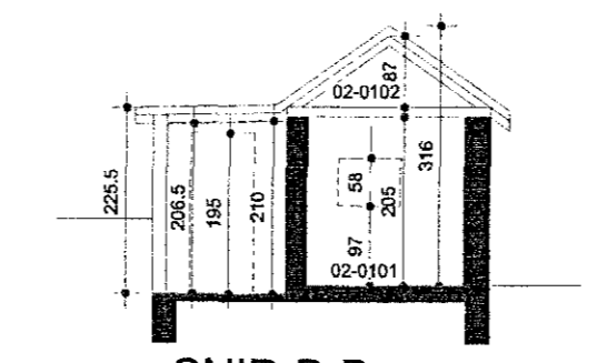
SNID B-B
