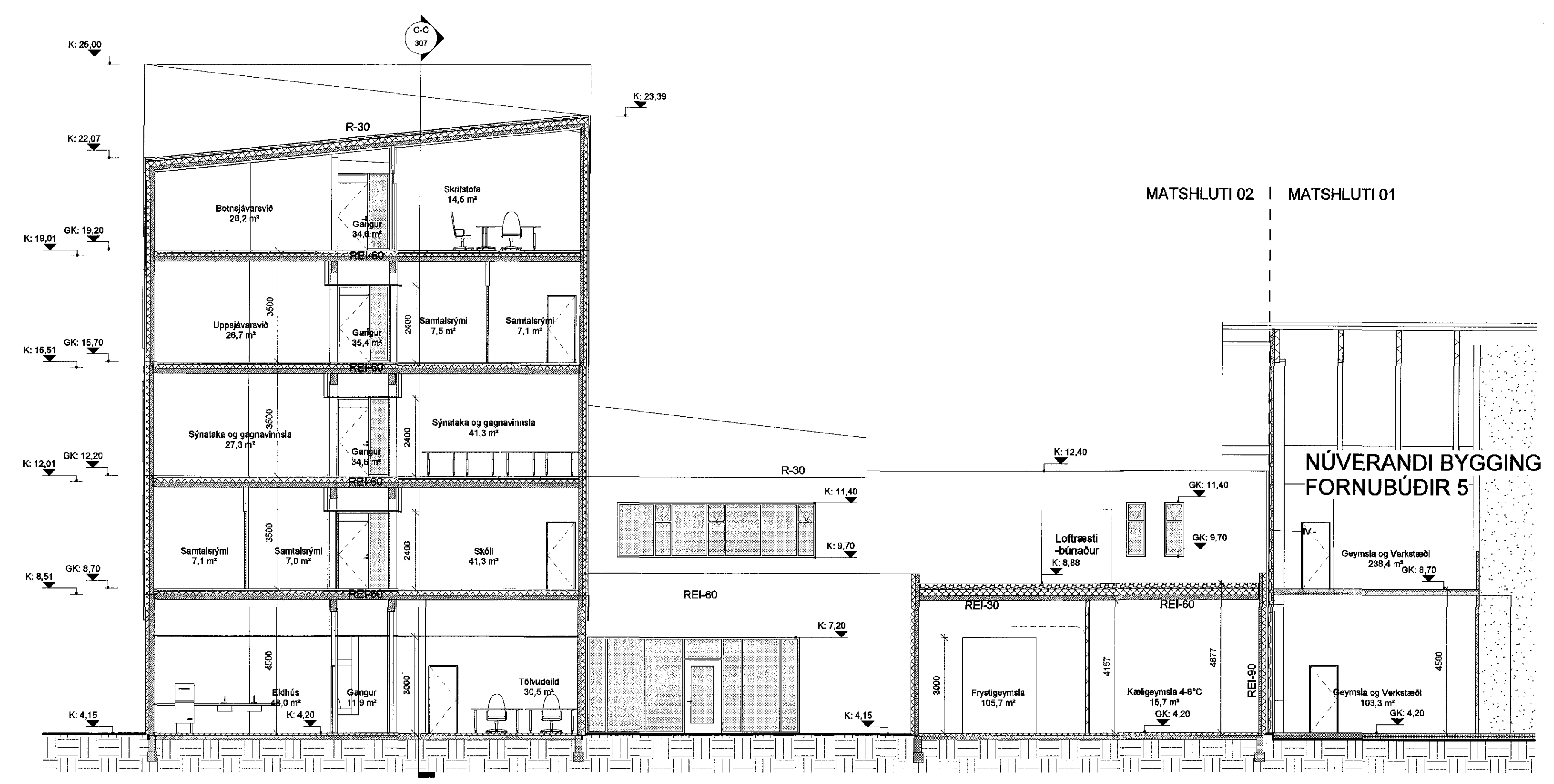
SNIB B-B
