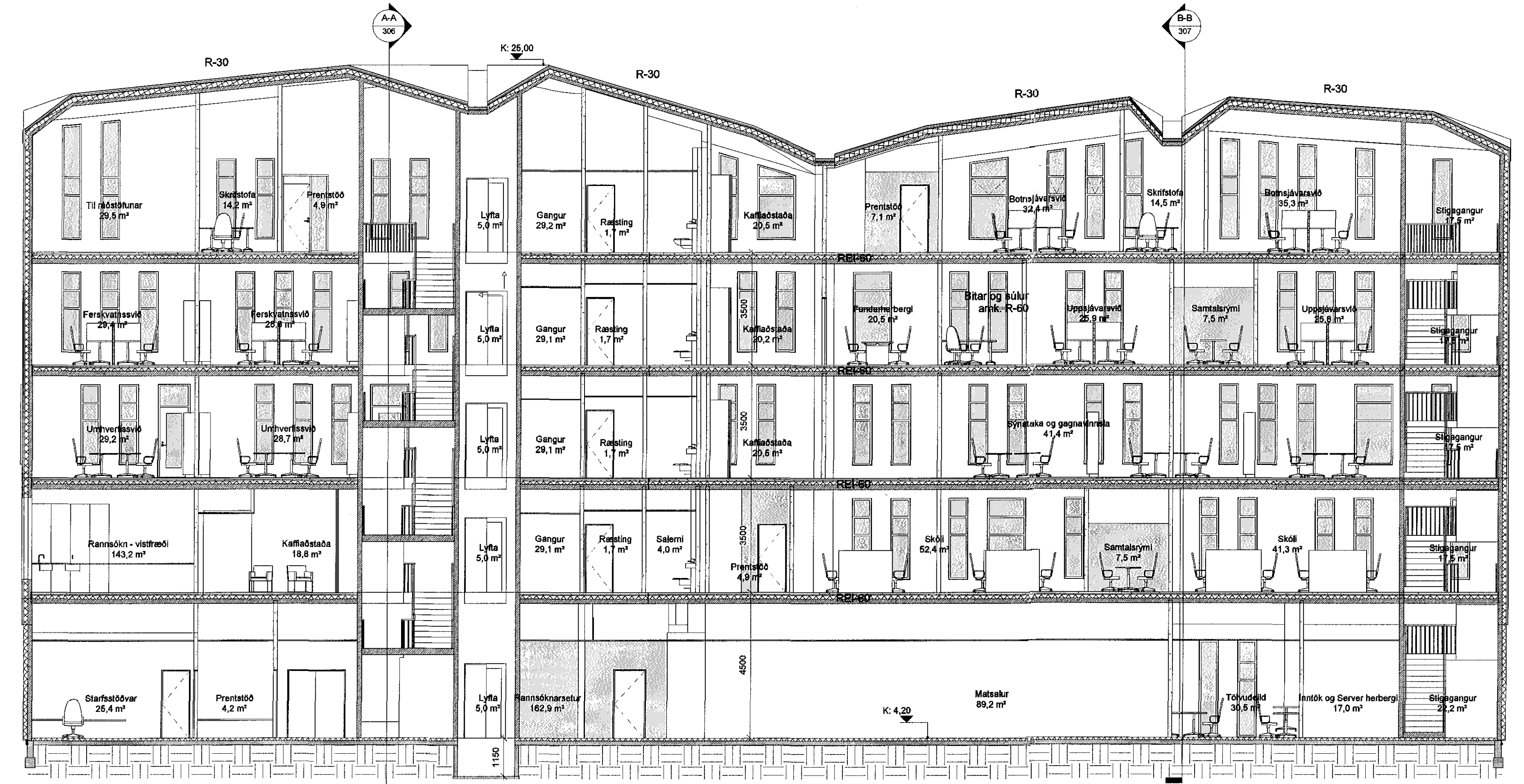
SNIB C-C
