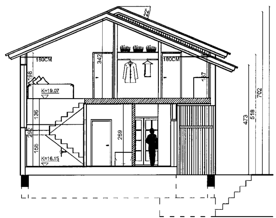
SNID A - A 1:100
