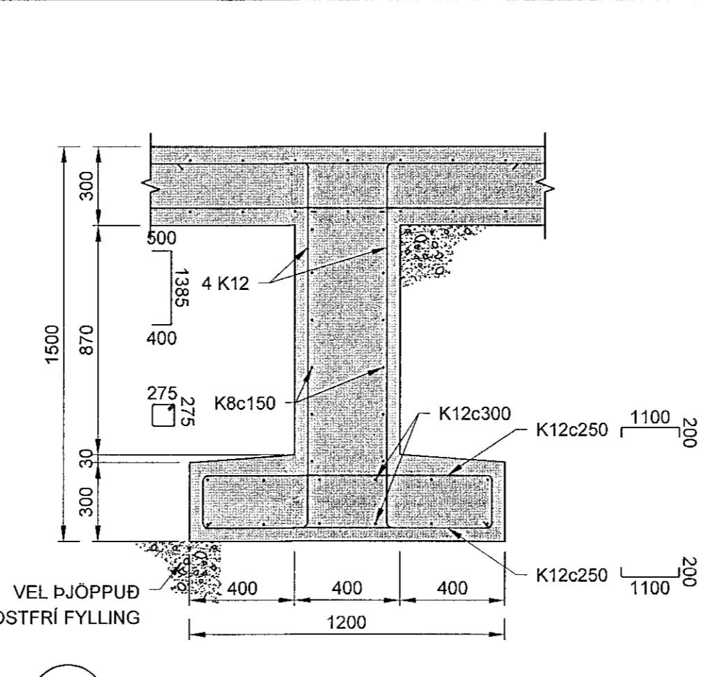
9 SNID 1:20
