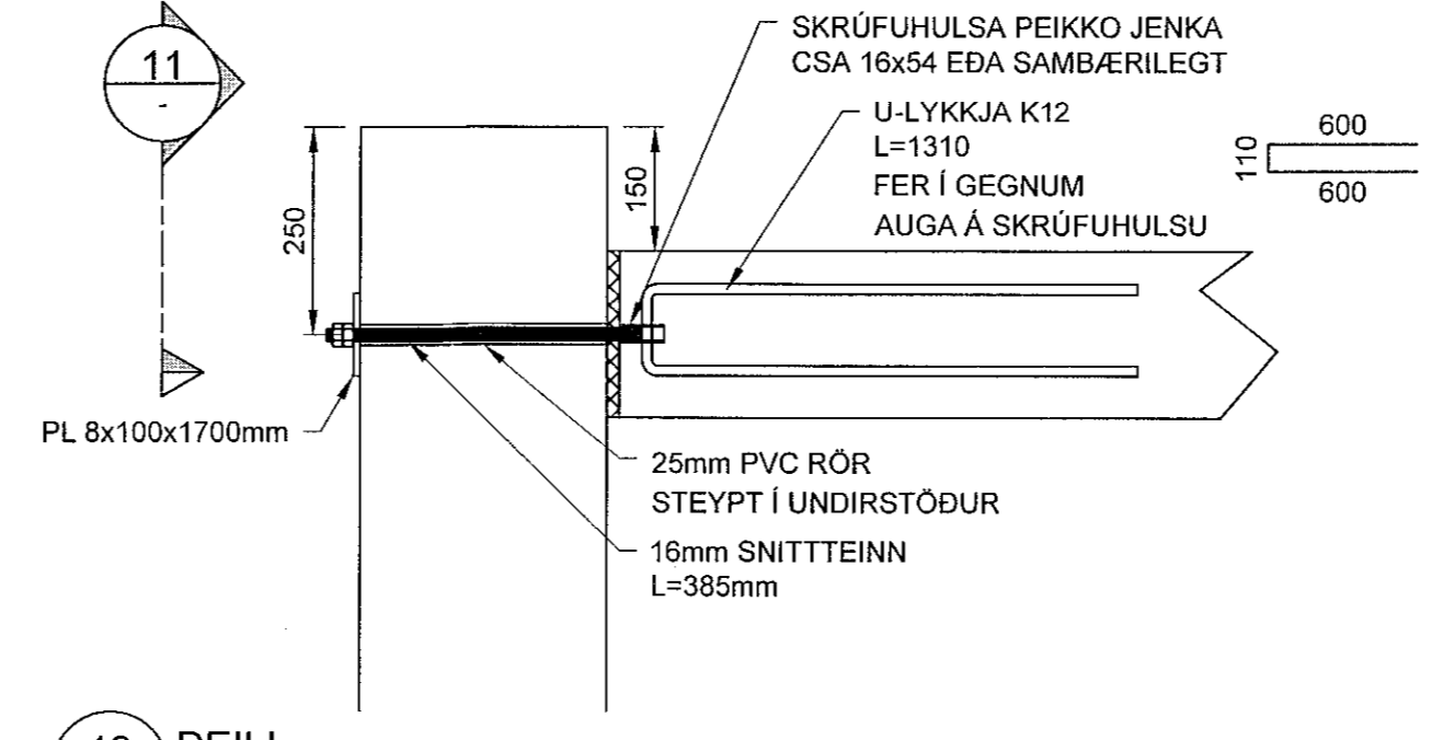
11 SNID 1:10
