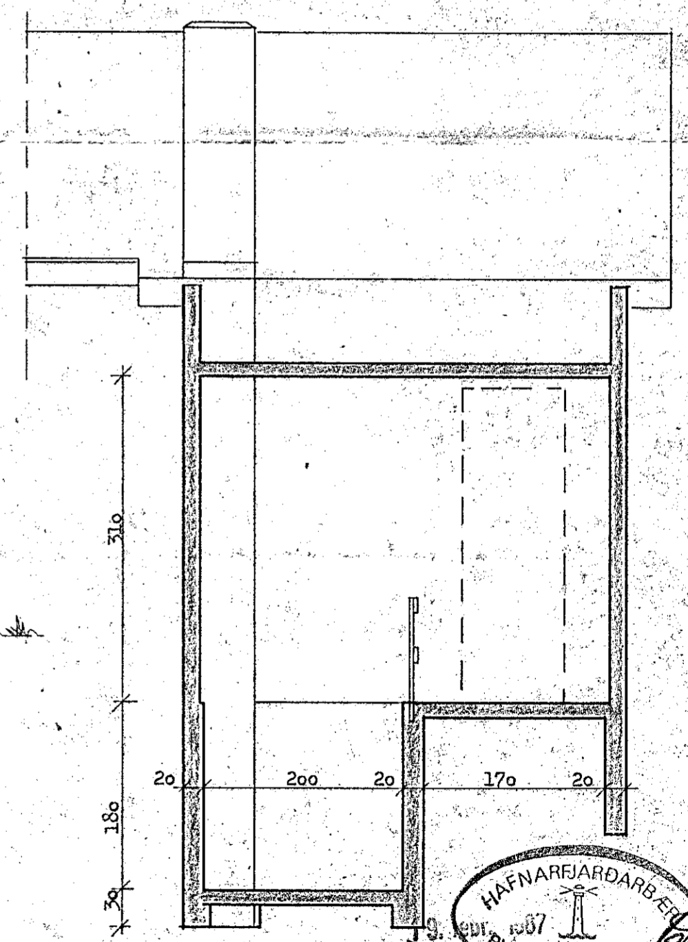
SNID C - C 1:50
