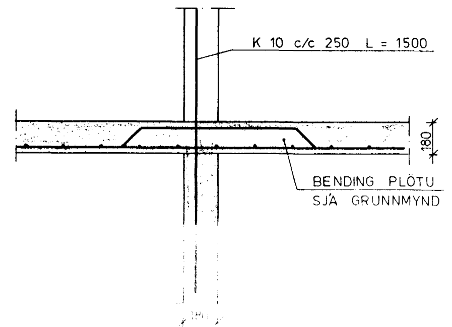
SNID C 1:20
