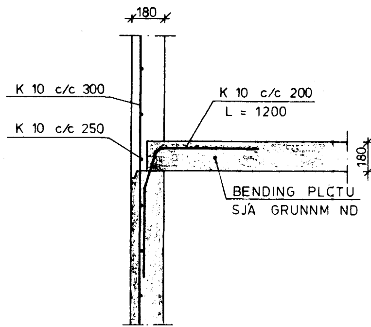
SNID A 1:20
