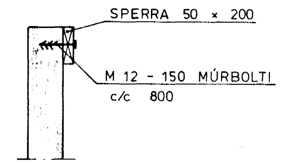
SNID B 1:20
