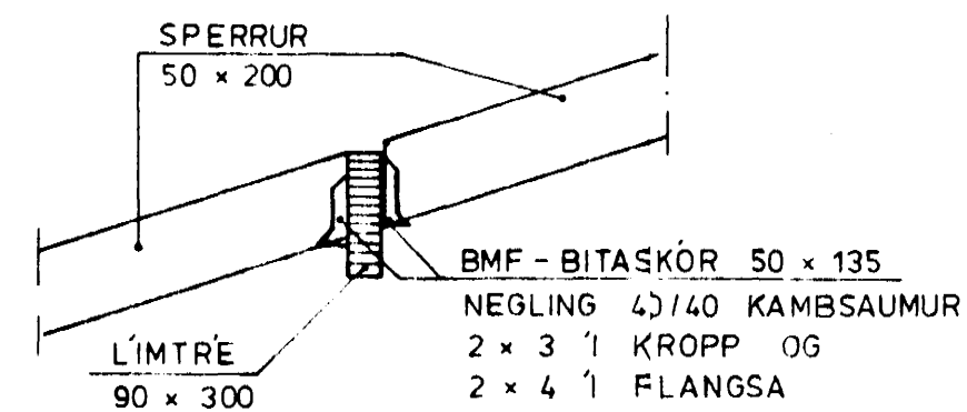
SNID C 1:20
