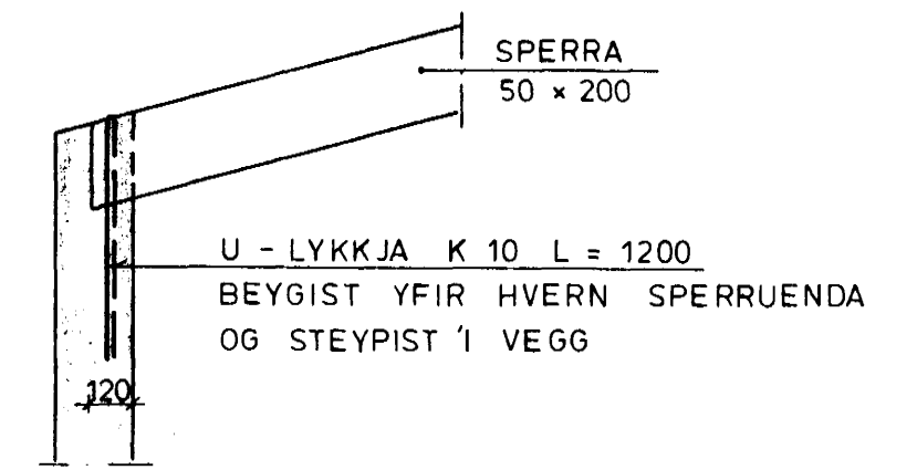
SNID A 1:20
