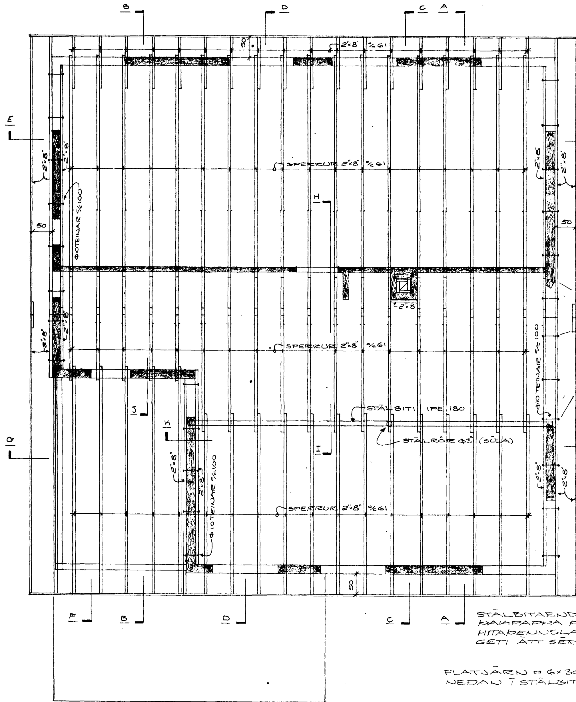
GRUNDMYND, M=1:850
