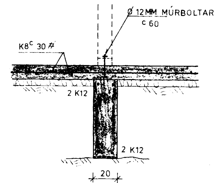
SNID 4-4 1:20
