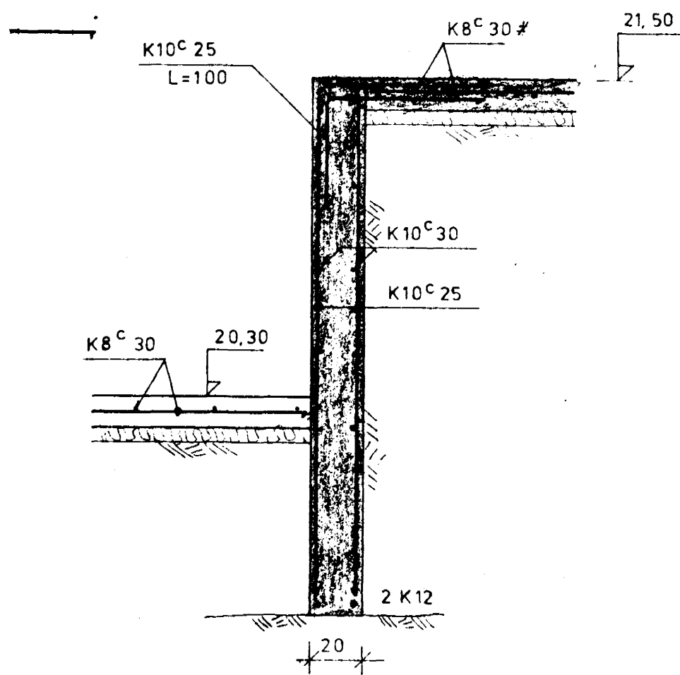
SNID 5-5 1:20
