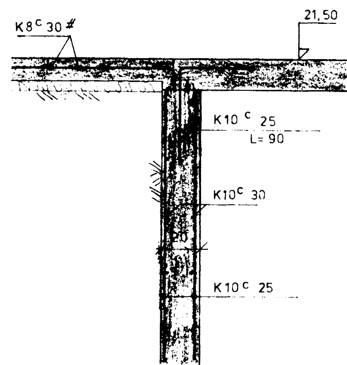
SNID 6-6 1:20
