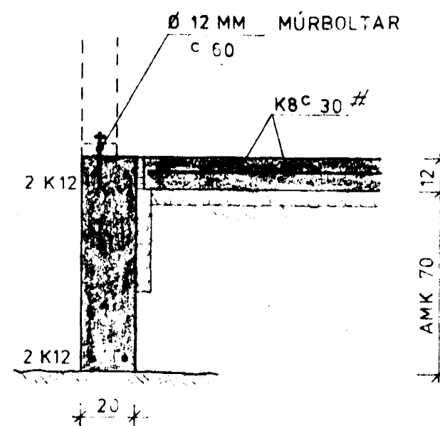
SNID 3-3 1:20
