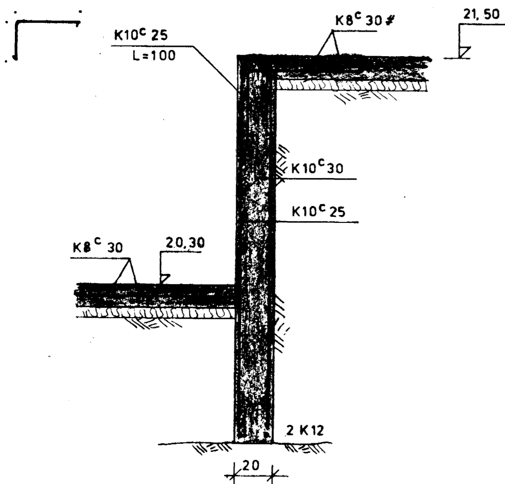
SNID 5-5 1:20
