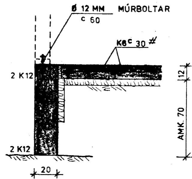
SNID 3-3 1:20
