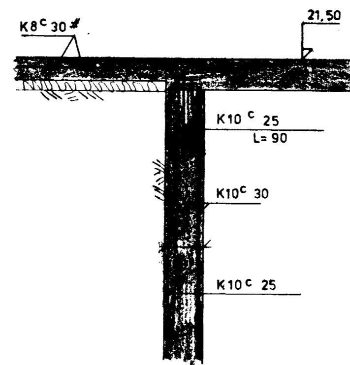
SNID 6-6 1:20
