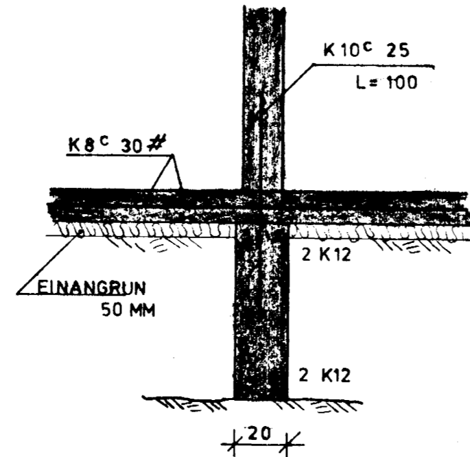
SNID 2-2 1:20
