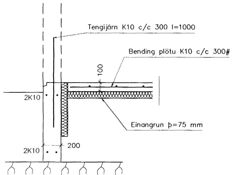
SNID 1, 1:20
