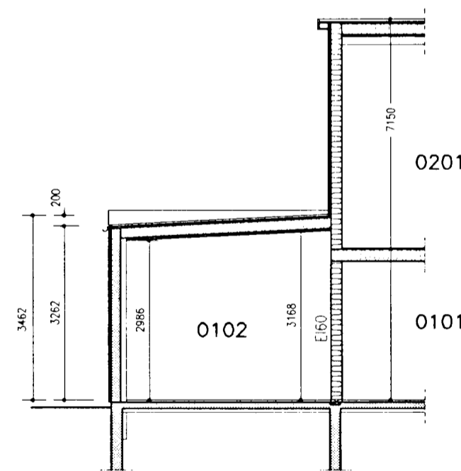
SNID 2-2 1:100
