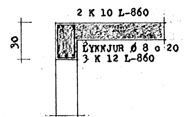
SNID - A 1:20
