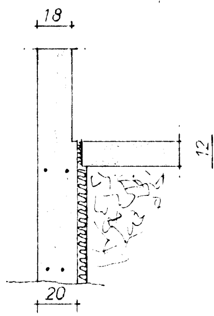
SNID A
