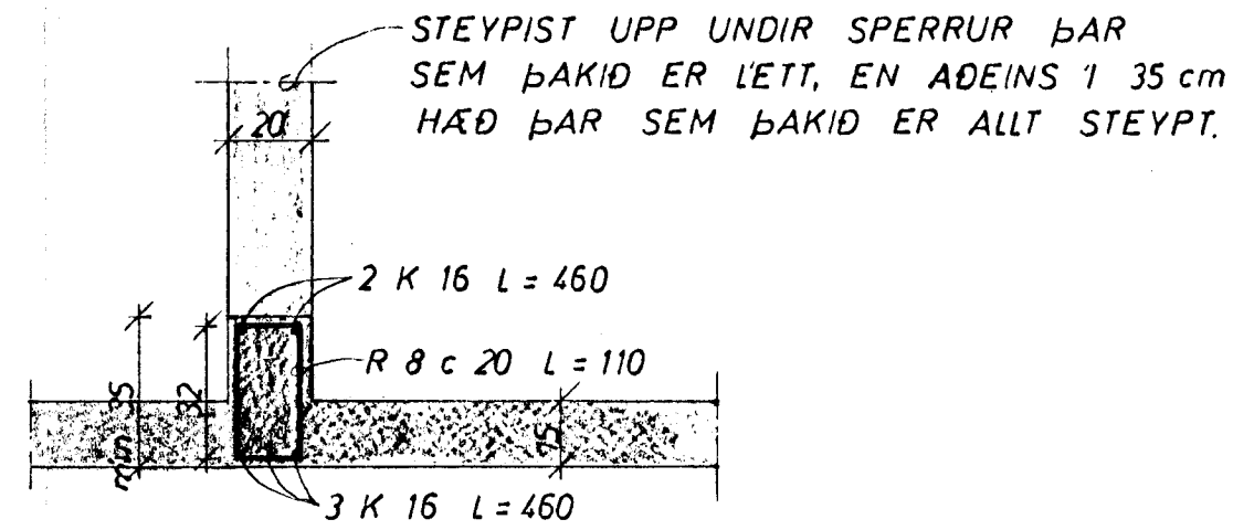
SNID A 1:20
