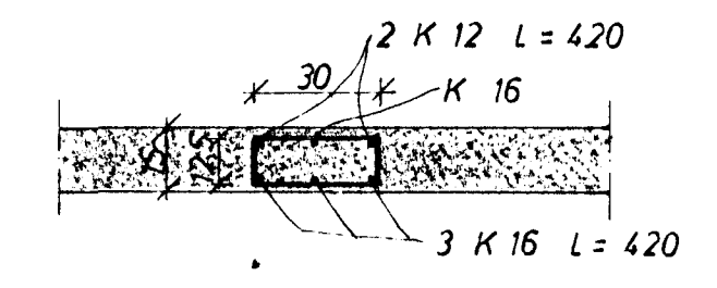
SNID C 1:20
