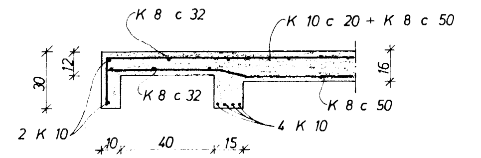
SNID A 1:20
