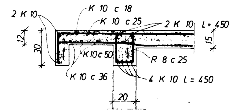
SNID A 1:20
