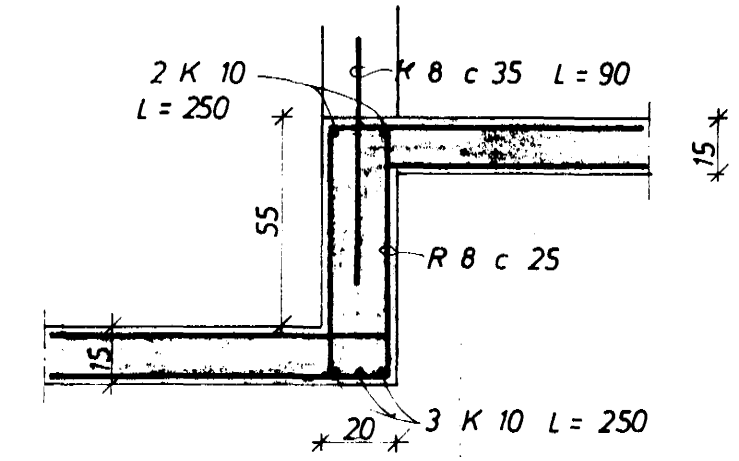
SNID B 1:20
