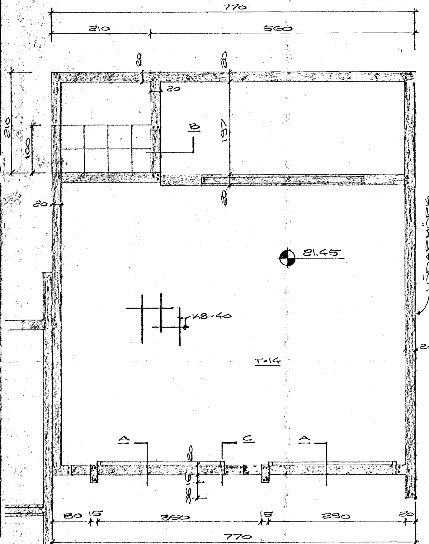
DAKPLATA GRUNDMYND, M=1:850
