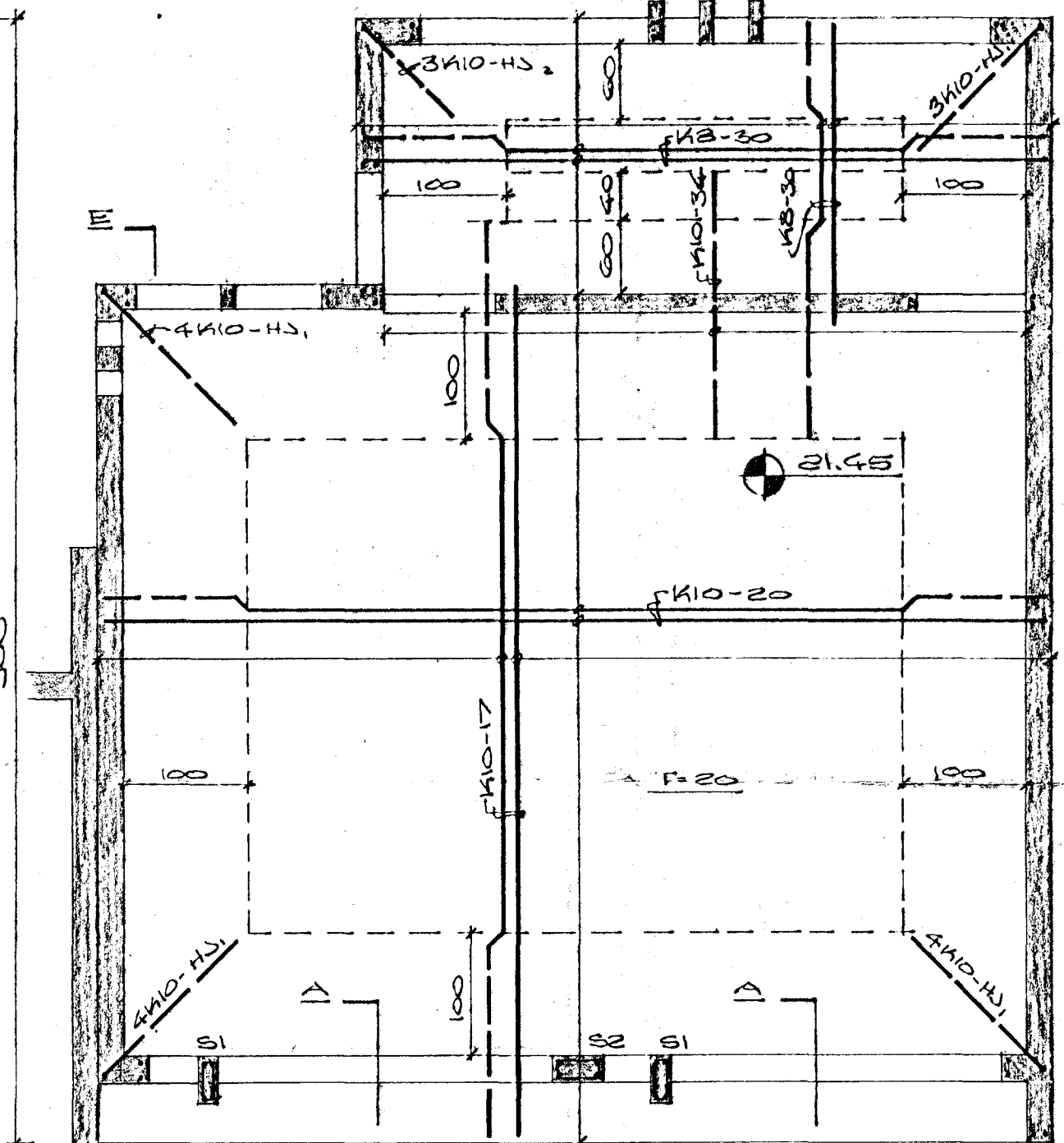
DAKPLATA GRUNDMYND, M=1:850
