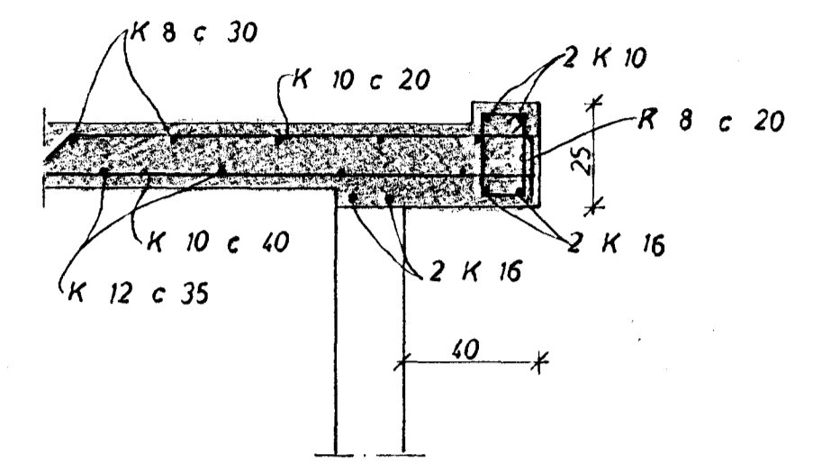
SNID A 1:20
