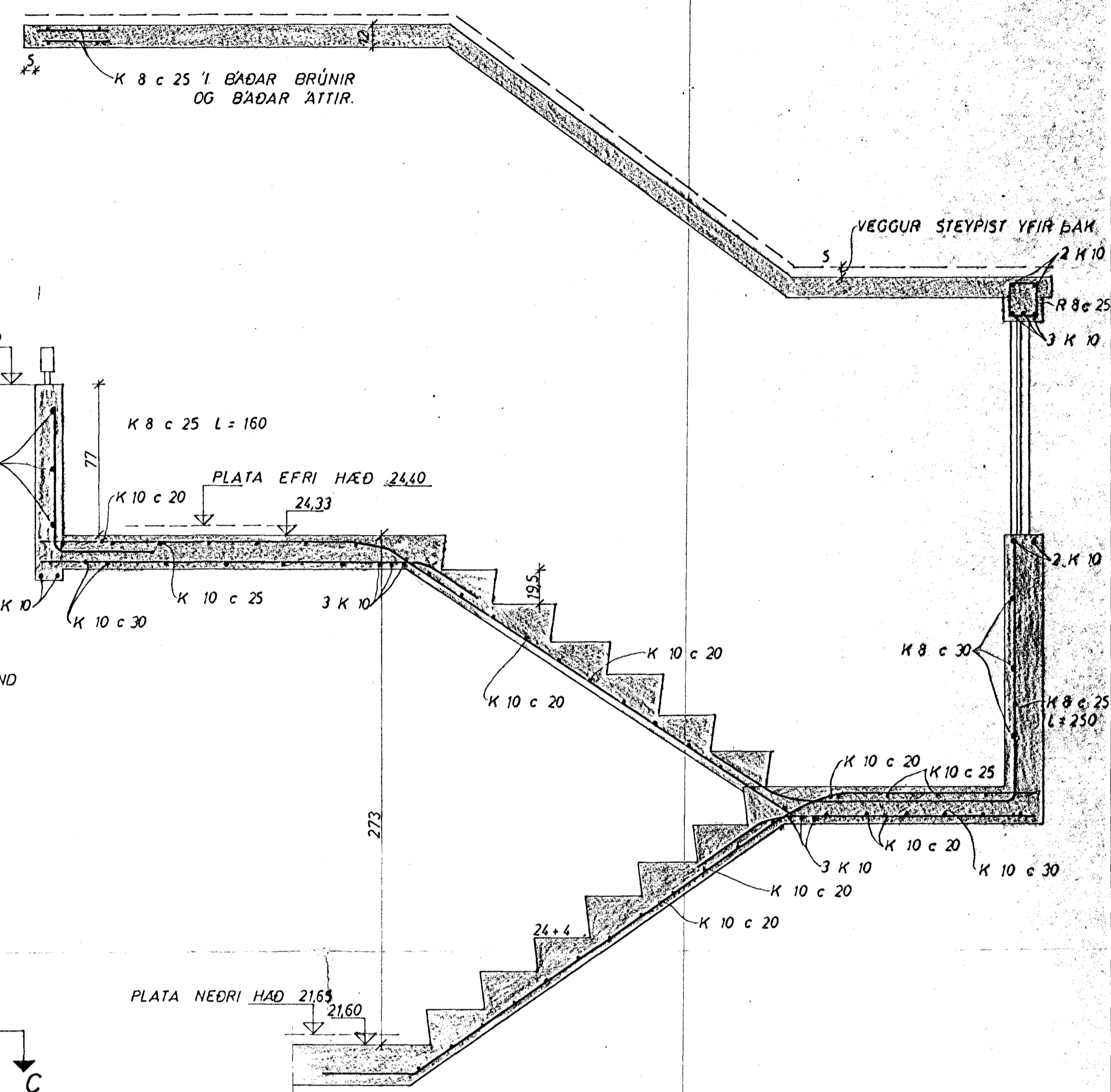
SNID B 1:20
