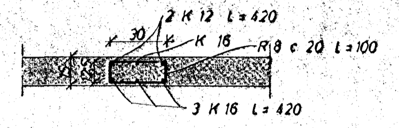
SNID C 1:20
