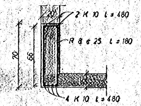
SNID B 1:20
