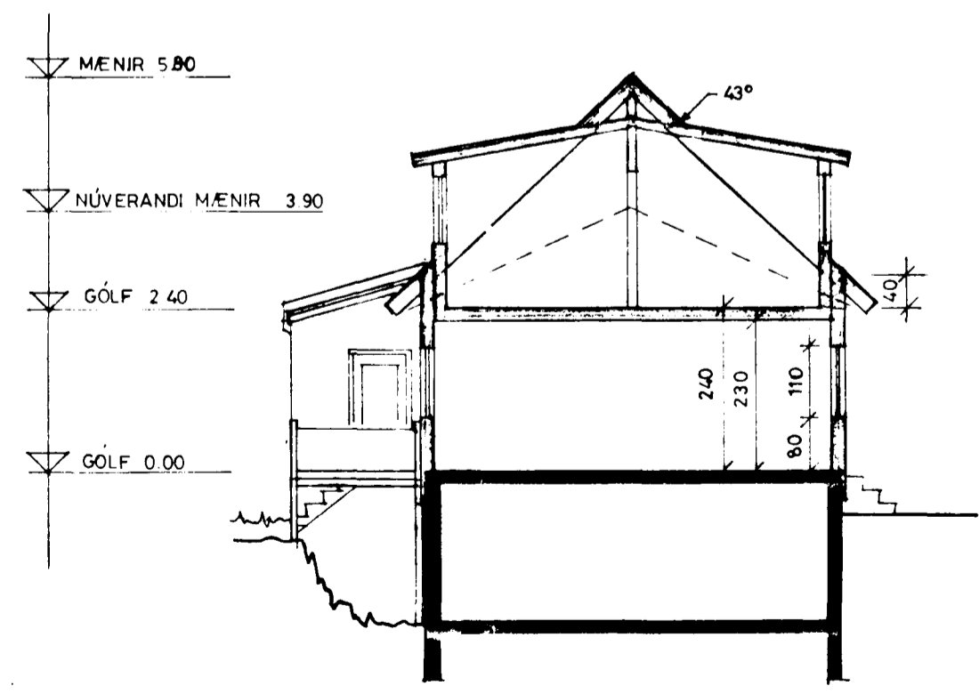
SNID 1:100
