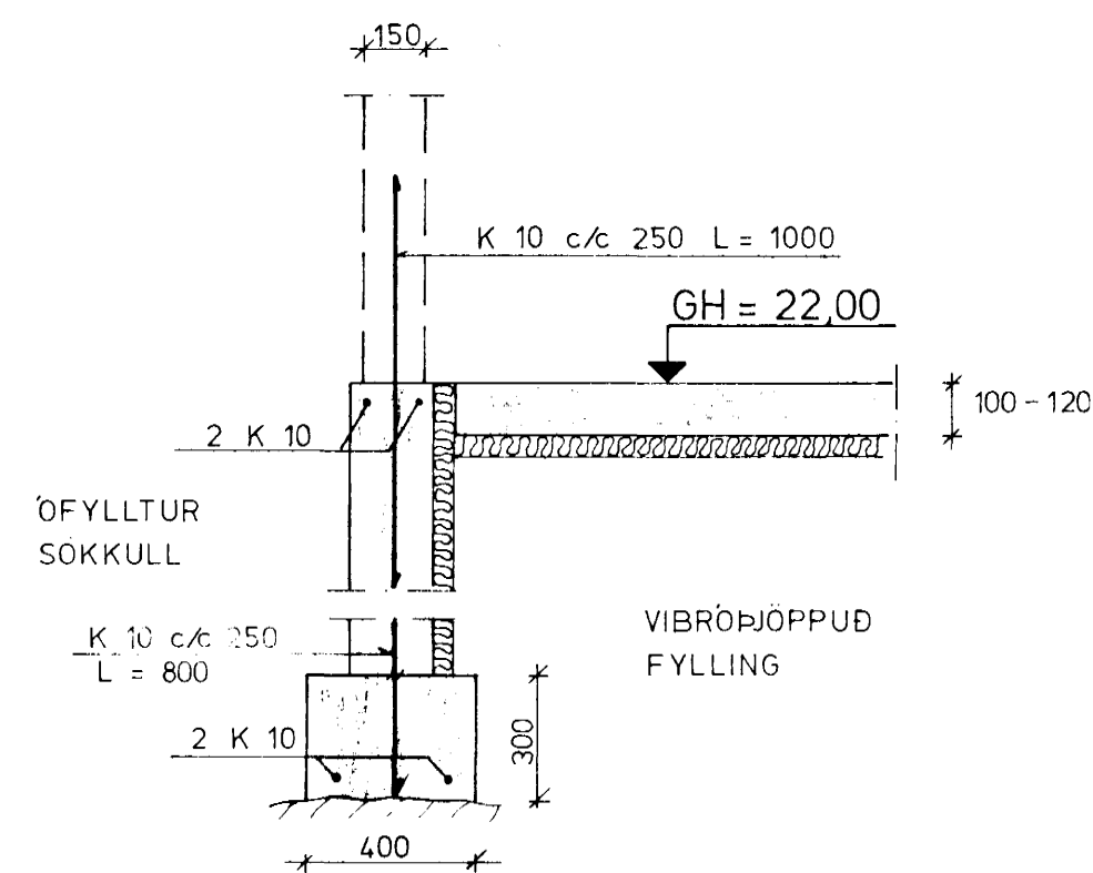
SNID C 1:20
