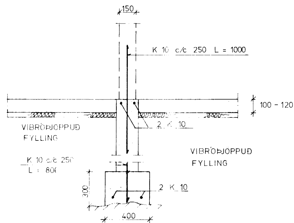
SNID B 1:20
