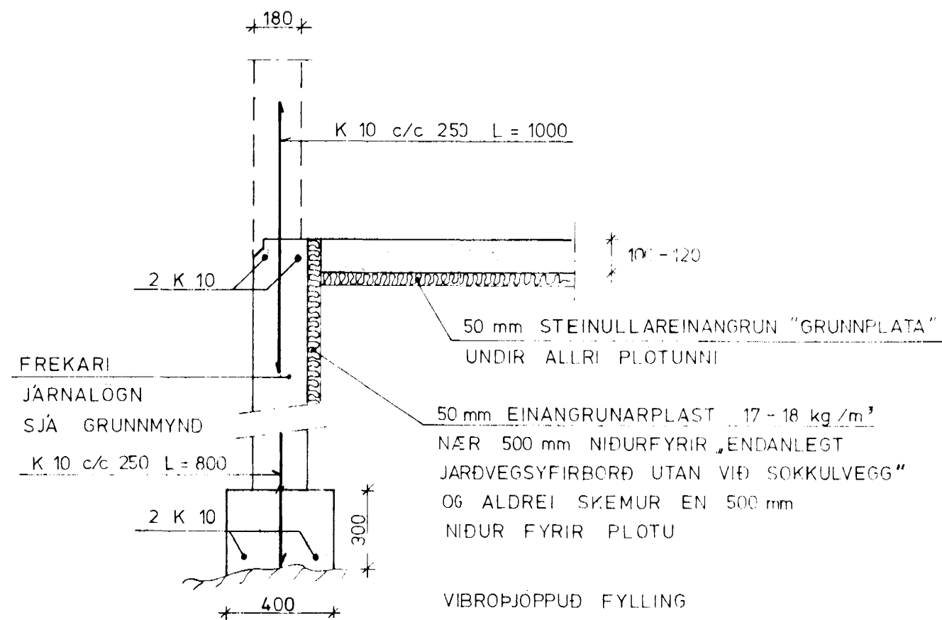
SNID A 1:20
