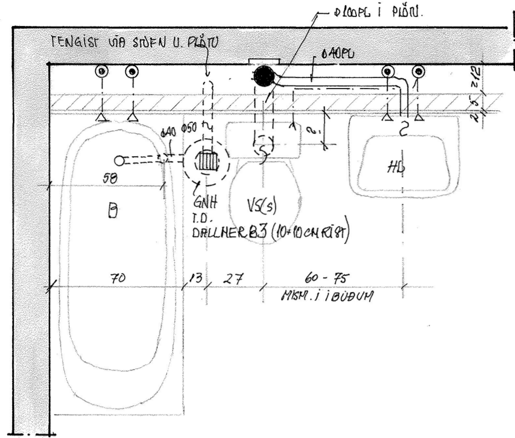
SNYRTING: HLIDARM. 1:20.
