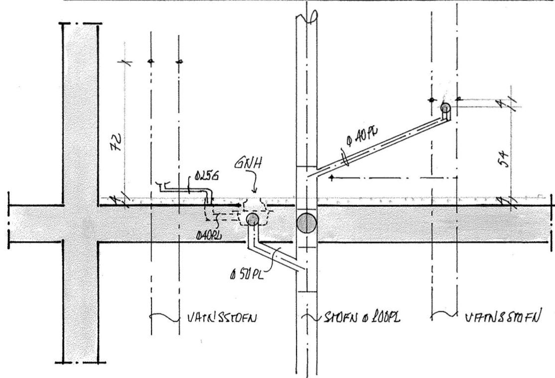
SNYRTING: HLIDARM. 1:20.
