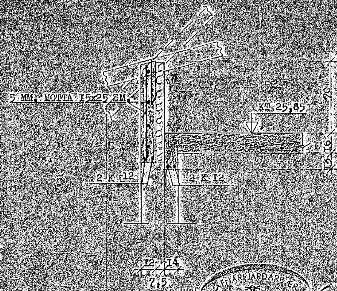
SNID F-F 1:20
