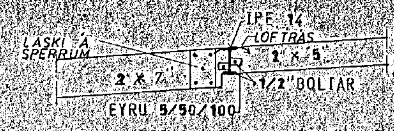
SNID C 1:20
