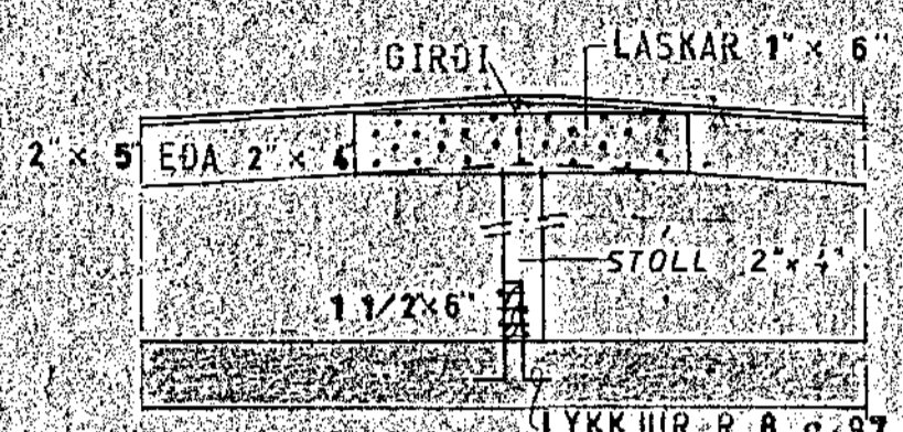
SNID F 1:20
