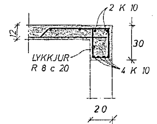
SNID C 1:20
