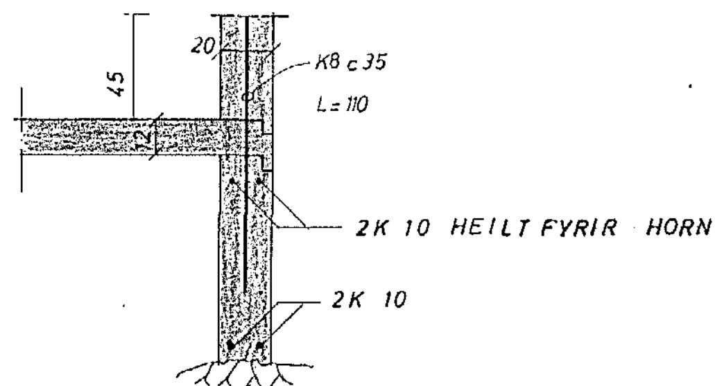
SNID A 1:20
