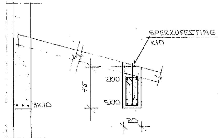
SNID A - A 1:20
