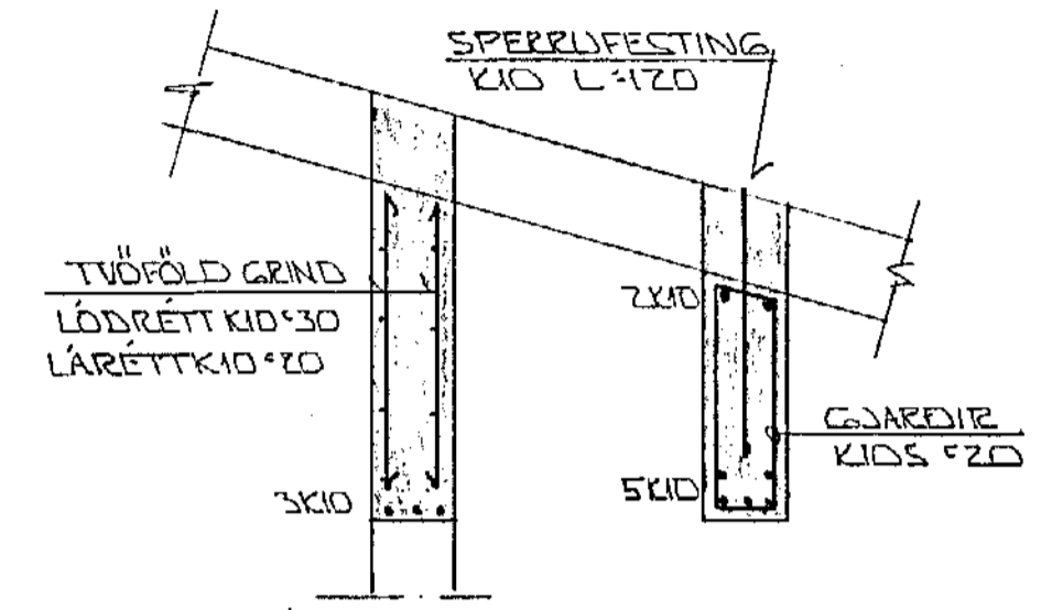
SNID 8-8 1:20
