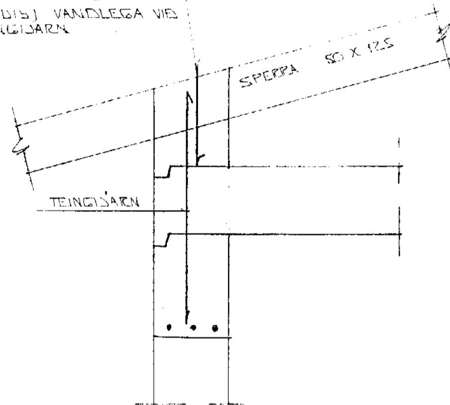
SNIED 7 - 1:10
