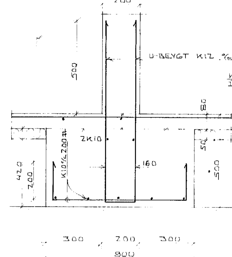
SNID C-C 1:10
