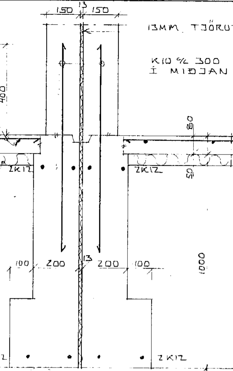
SNID C-C 1:10
